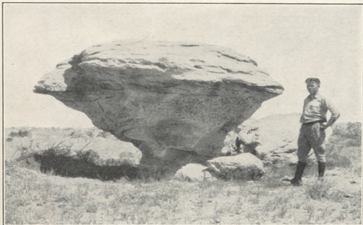
B. PEDESTAL ROCK OF SANDSTONE NEAR MCGILLVRAY'S RANCH, MCKINLEY COUNTY, N. MEX.
