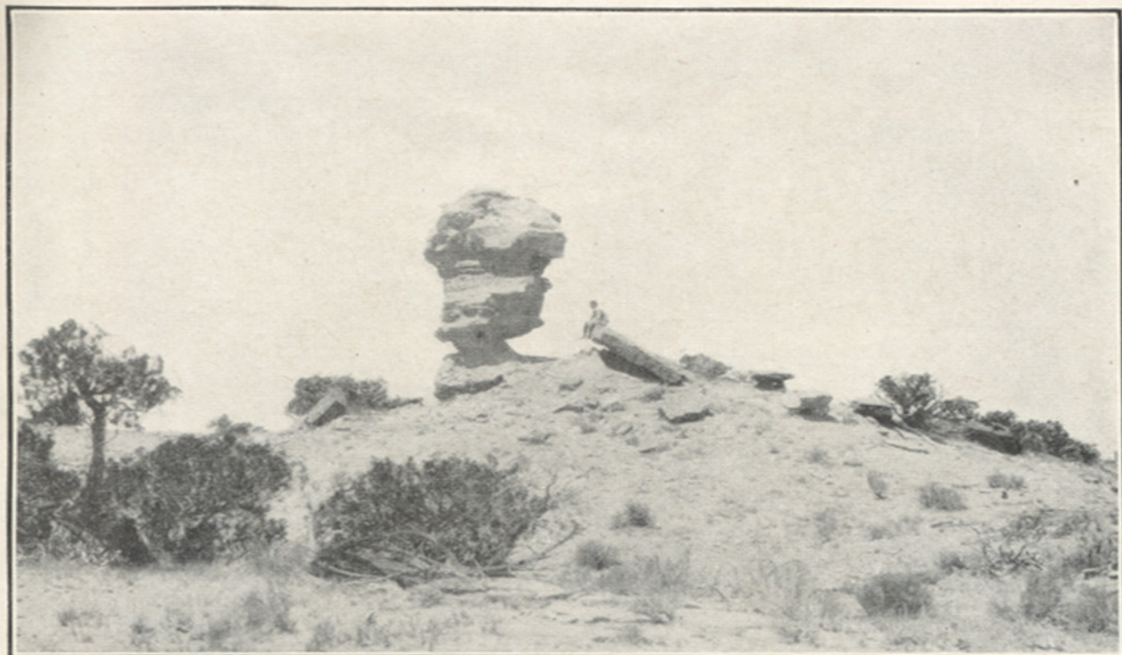
A. PEDESTAL ROCK OF SANDSTONE NEAR SEVEN LAKES, MCKINLEY COUNTY, N. MEX.
