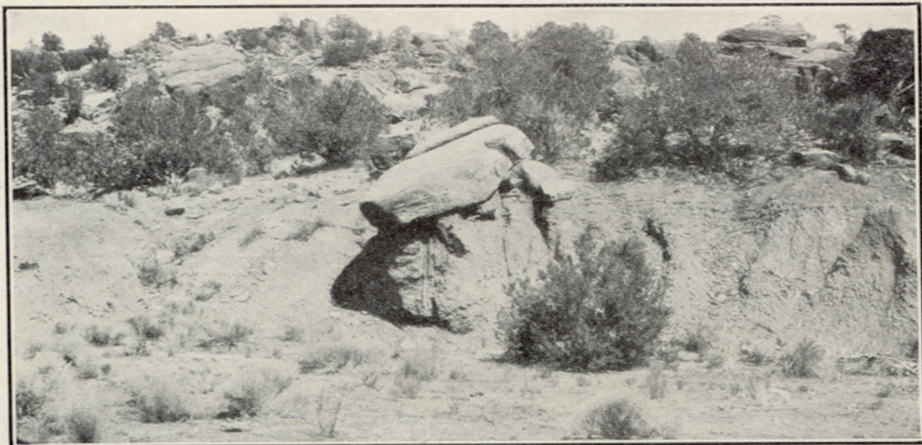
A. SANDSTONE BLOCK RESTING ON PEDESTAL OF SHALE DETACHED FROM THE BANK OF WHICH IT ONCE FORMED A PART
