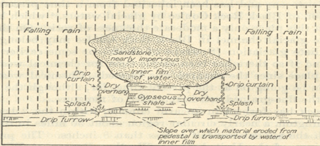
FIGURE 1.—Diagram illustrating differential rainwash on a pedestal rock consisting of an impervious block resting on an easily eroded mass below
