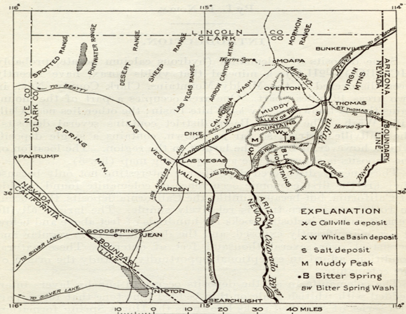
FIGURE 3.—Map showing location of colemanite deposits in Clark County, Nev.
