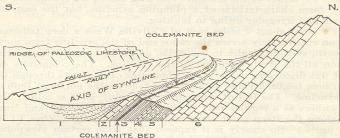
FIGURE 4.—Diagrammatic sketch showing mode of occurrence of colemanite deposit near Callville Wash, Clark County, Nev. Numbers correspond to those in section below.
