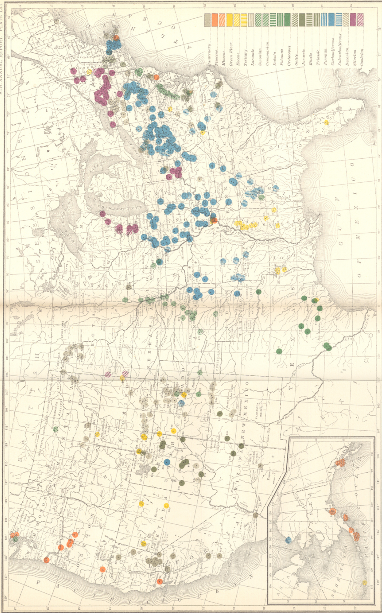
GEOGRAPHIC DISTRIBUTION OF FOSSIL PLANTS IN THE UNITED STATES. BY LESLIE F. WARD.
